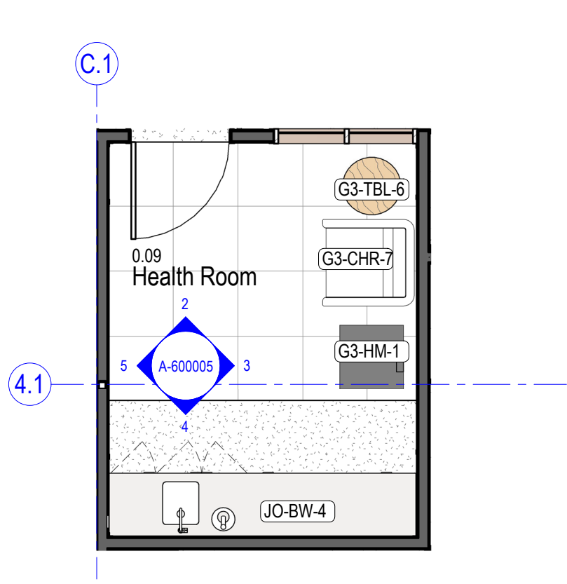
1 0.09 - Health Room - Plan 1 : 50
