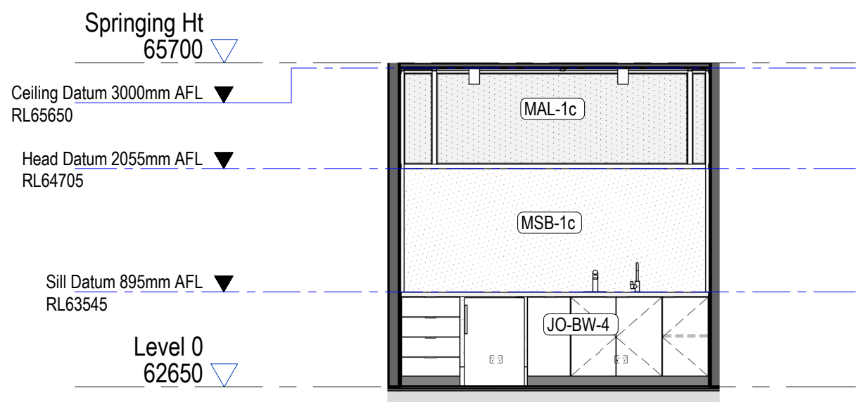
4 0.09 - Health Room - South Elevation 1 : 50
