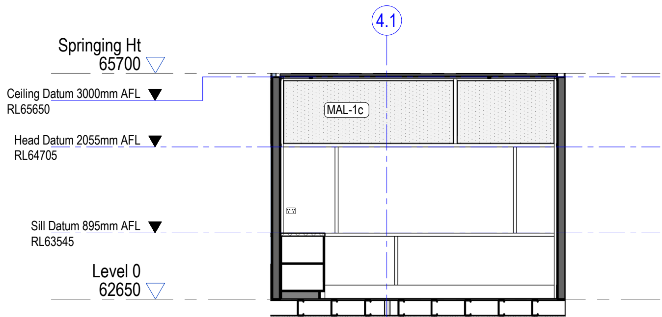
5 0.08 - Health Room - West Elevation 1 : 50
