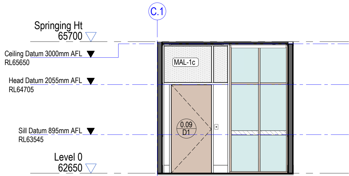
2 0.09 - Health Room - North Elevation 1 : 50
