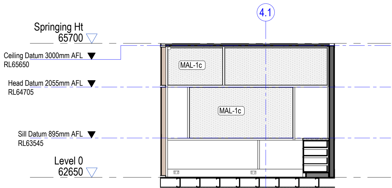
3 0.09 -Health Room - East Elevation 1 : 50
